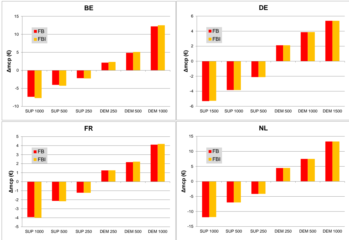
Figure 6 Resilience per bidding area at 90% in €/MWh
