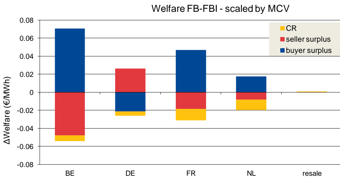
Figure 9 Distribution of DA market welfare per area scaled by market clearing volume
