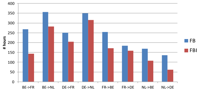
# IDATC capacity < 100 MW (non-intuitive hours only)
