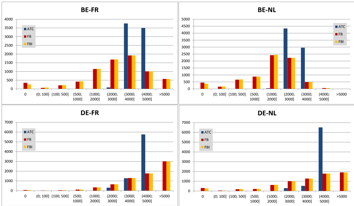
Figure 11 Histogram of ID capacity per border (sum of both directions). Vertical axes contain frequencies in number of hours.
